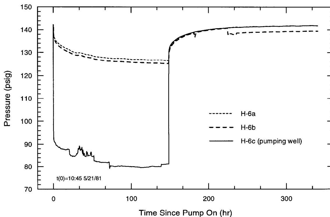
Figure 5-4. Pressures during H-6 pumping test #3.
