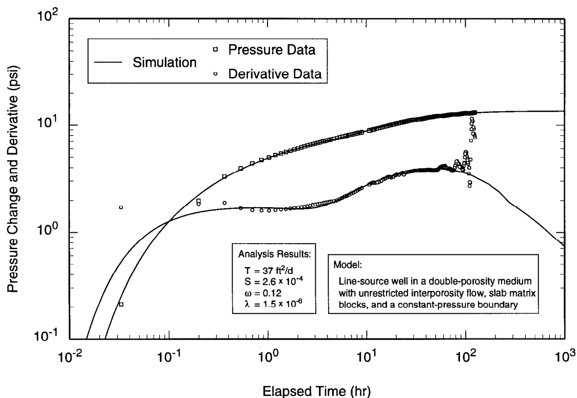
Figure 6-16. Log-log plot of H-6a recovery data from test #2 with Interpret/2 simulation.
