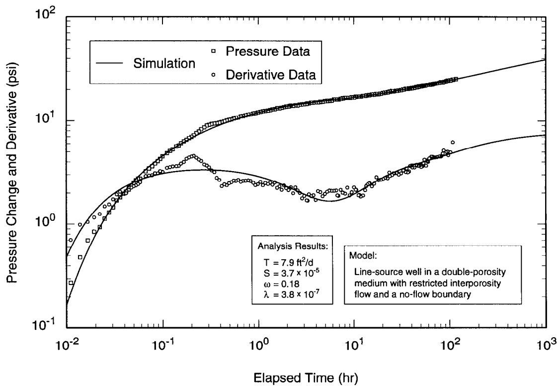
Figure 6-90. Log-log plot of H-19b6 drawdown data with Interpret/2 simulation.
